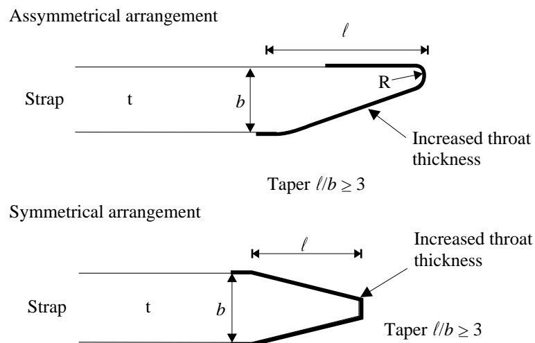
Fig. 6.6 Termination of straps
