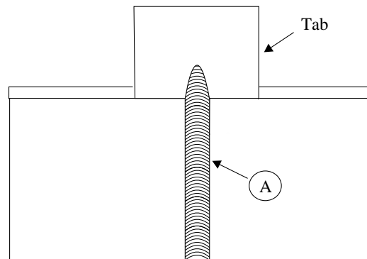
Fig 6.8.b End crack termination
